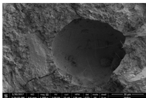
SEM images of an open pore in plan cement paste without any crystalline waterproofing treatment
